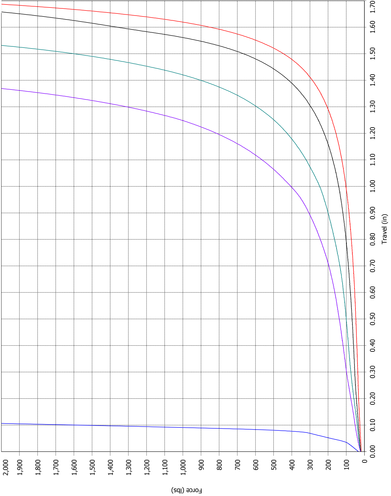
Force vs. Travel
